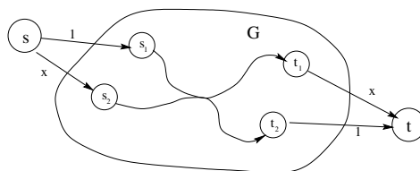
Figure 6: Proof of Theorem 3.17. In a “no” instance of 2DDP, the existence of s_1-t_1 and s_2-t_2 paths implies the existence of an s_1-t_2 path.
